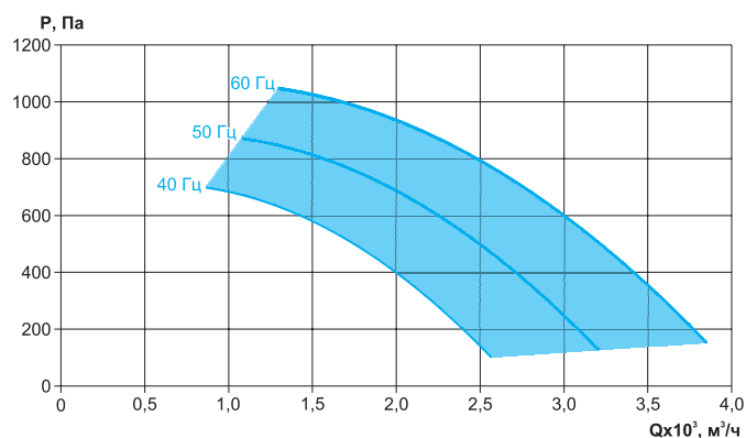
ВРС-К-60-35/28-РЦ-1,1/3000/220-380
