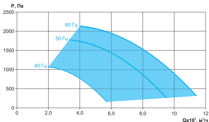
VCB-LT-630-O/40-РЦ-4,0/3000/220-380-Y2
