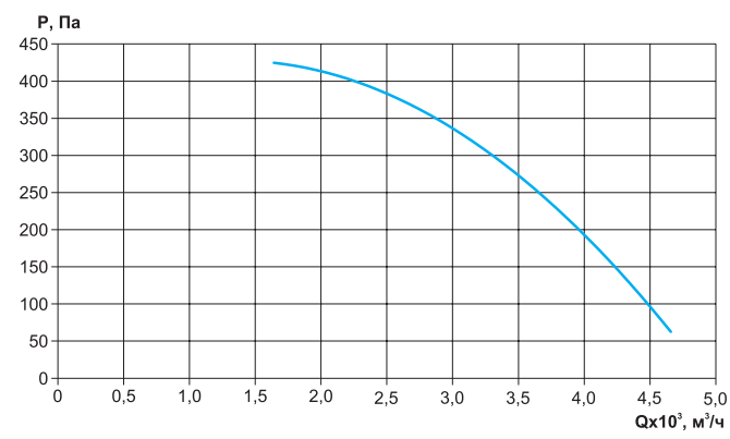
VCB-LT-400-O/40-ПЦ-0,75/1500/220-Y2
