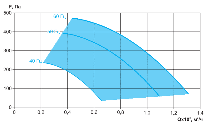
VCB-LT-315-O/20-РЦ-0,25/3000/220-380-У2
