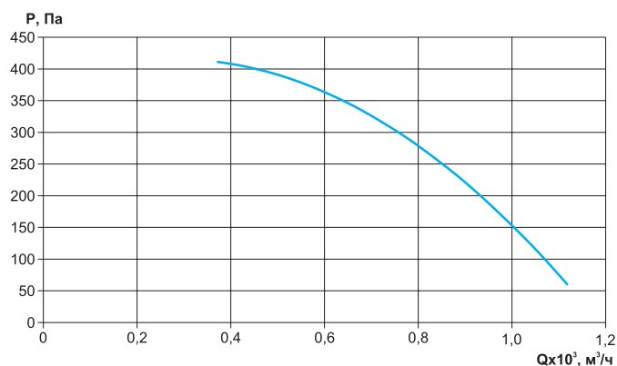
VCB-LT-315-O/20-ПЦ-0,25/3000/220-У2
