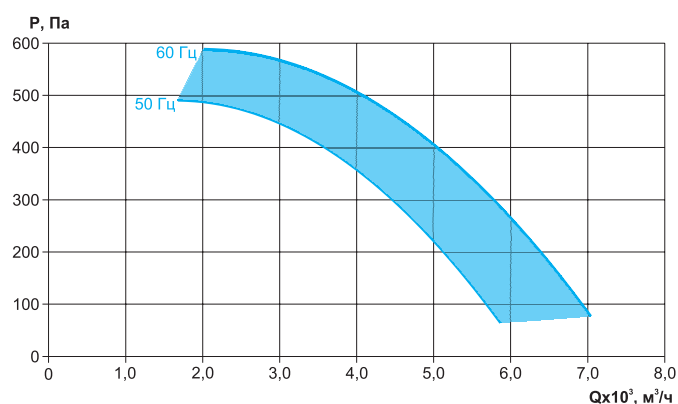
ВРС-К-100-50/45-РК635-1,5/1500/220-380
